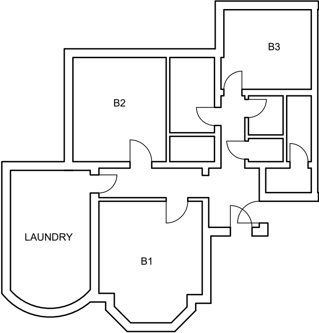
BASEMENT PLAN
